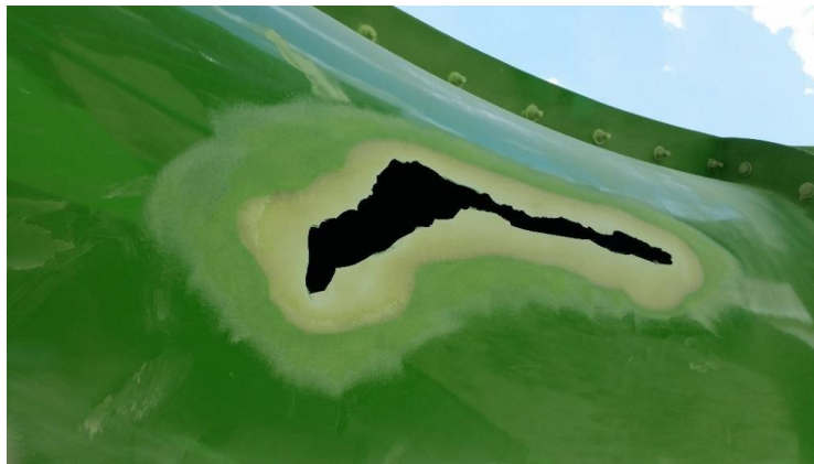
Figure 30: Grind and Sand Edges of Repair Area
